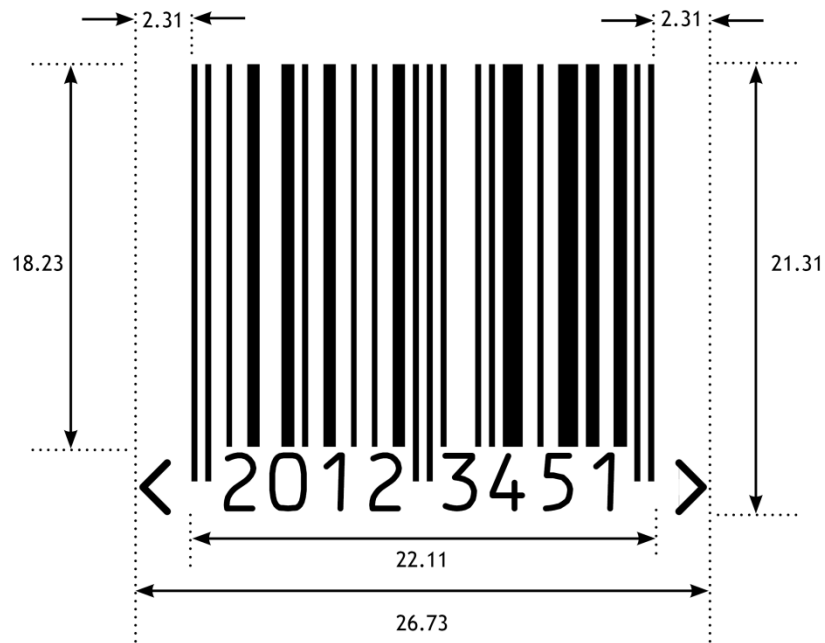
Figure 5.2.6.6-4. UPC-E barcode
